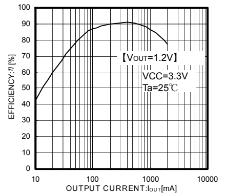
Fig.19 Efficiency
