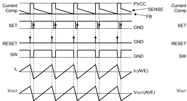
Fig.22 PWM switching timing chart
