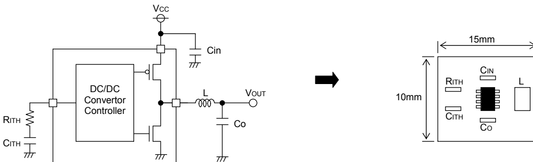
Fig.20 Example application
